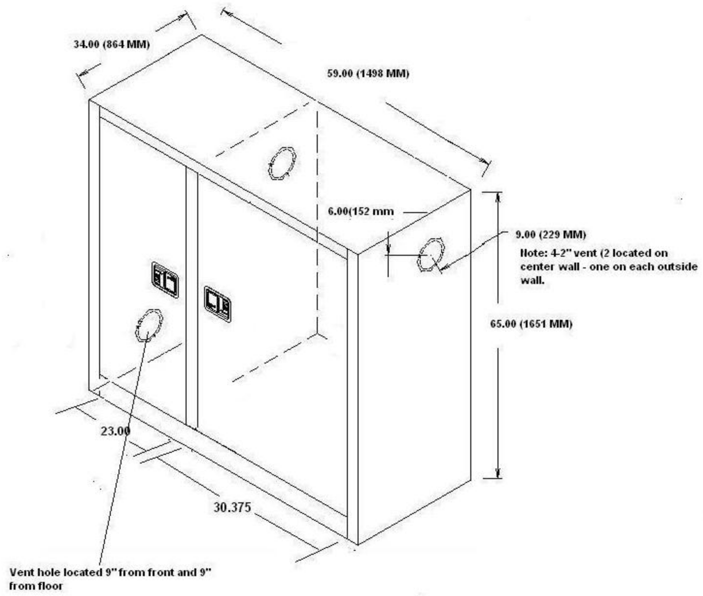
Double-Duty Storage Cabinet (Holds 1-30G (100L) or 1-55G(200L) and 12 5G safety cans)
